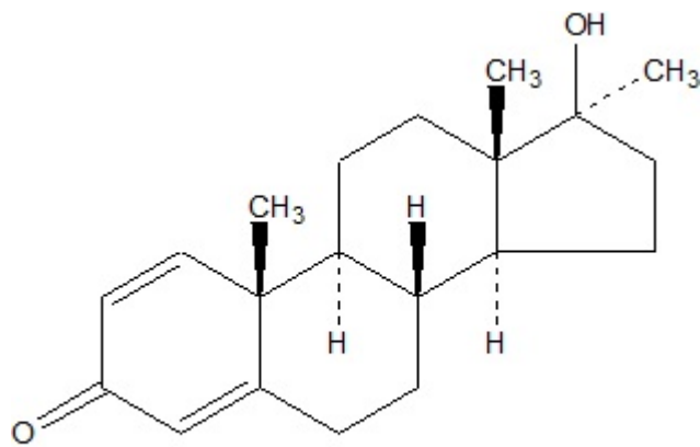
Methandienone
